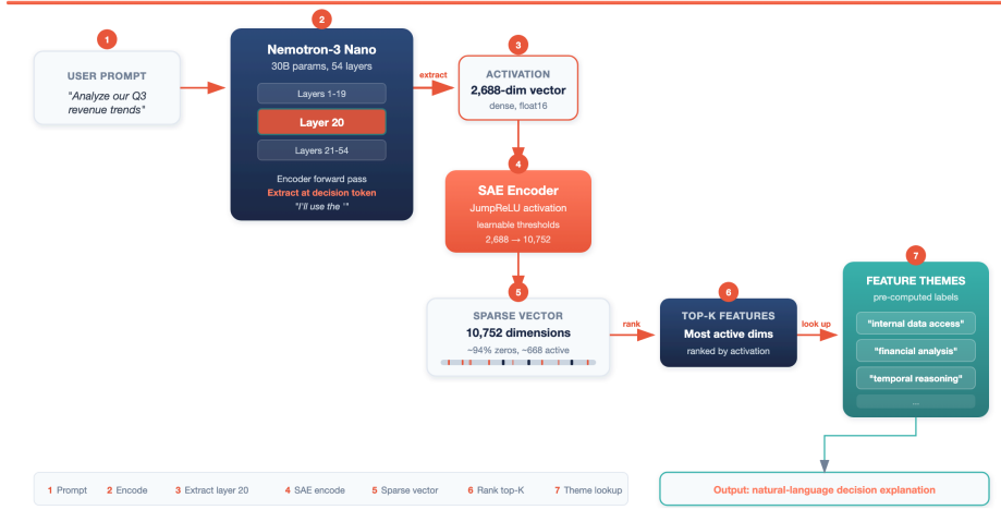
Fig. 5. Inference pipeline for real-time decision explainability. A user prompt is encoded by the Nemotron subject model; the hidden state at layer 20 is intercepted and projected through the trained SAE into a sparse 10,752-dimensional feature vector. The top-K active dimensions are mapped to pre-computed feature labels to produce a human-readable decision report.
