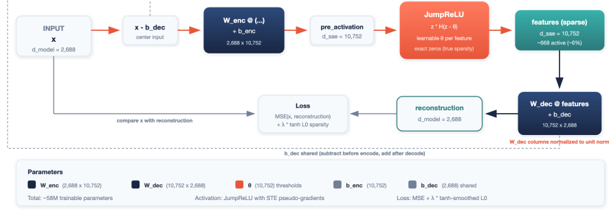
Fig. 4. JumpReLU Sparse Autoencoder architecture. The input activation \mathbf{x} is centered by subtracting \mathbf{b}_{\text{dec}} , projected to a 10,752-dimensional latent space via W_{\text{enc}} , and sparsified by the JumpReLU activation with learnable thresholds \theta . The decoder reconstructs via W_{\text{dec}} + \mathbf{b}_{\text{dec}} (shared bias). The loss combines reconstruction MSE with a smooth tanh-based L0 sparsity penalty.
